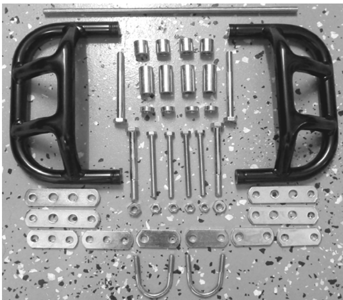
Universal Crash Bars
